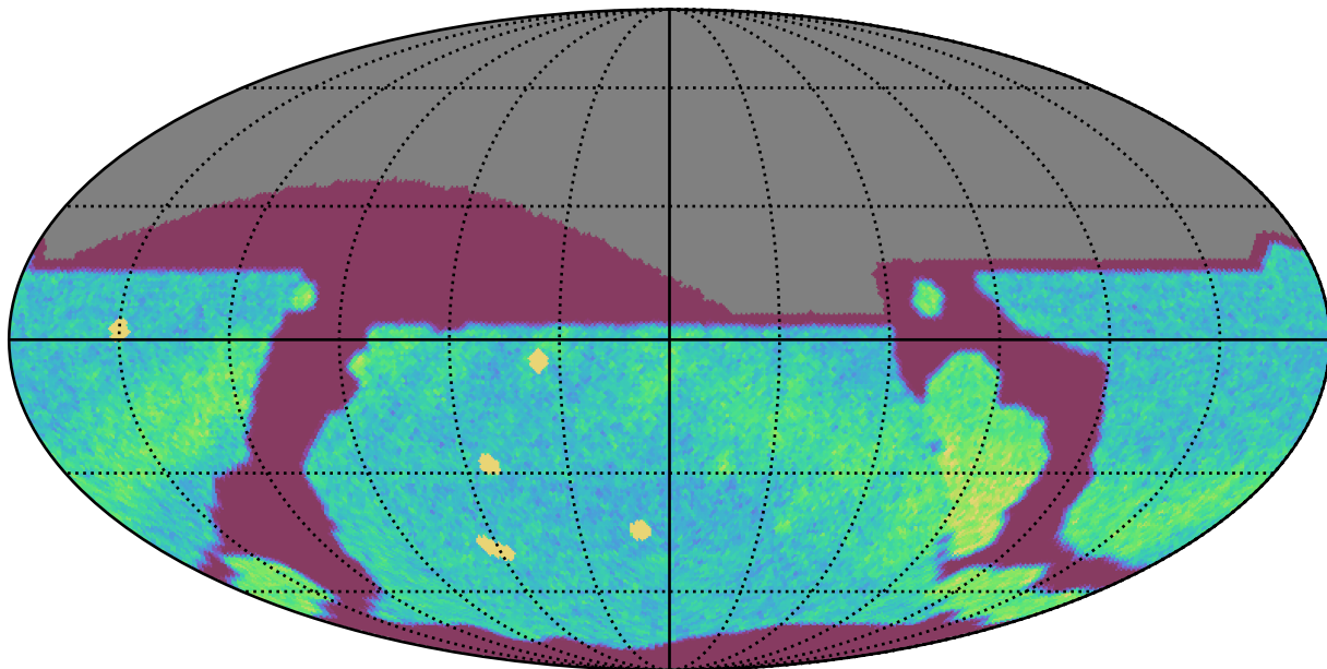
ddf_acor_sf20_lsf30_lsr20_v3.4_10yrs All sky r band: NVisits
