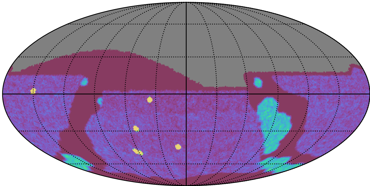
ddf_acor_sf20_lsf30_lsr20_v3.4_10yrs All sky g band: NVisits
