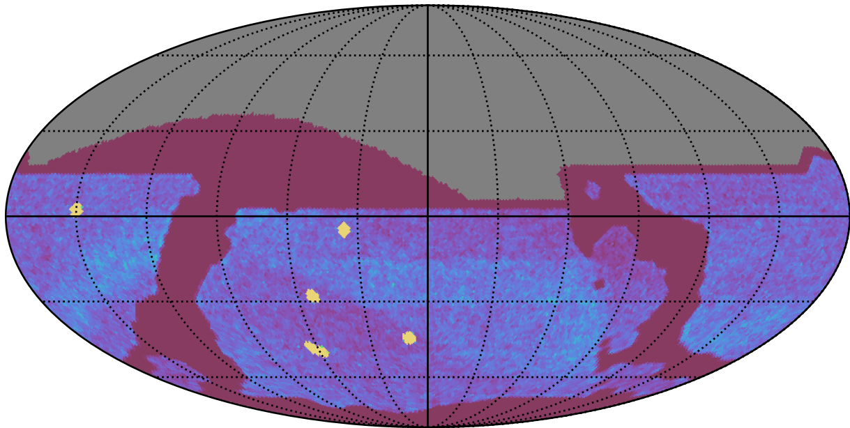
ddf_acor_sf20_lsf30_lsr20_v3.4_10yrs All sky all bands: NVisits
