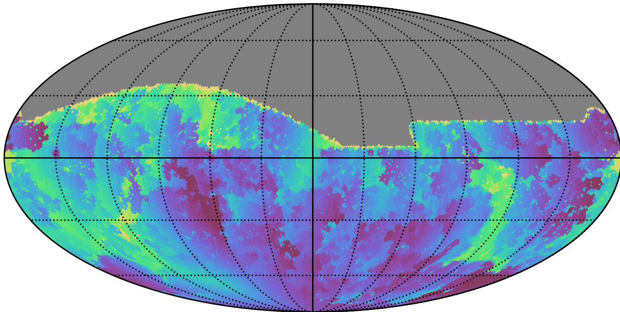
ddf_acor_sf20_lsf30_lsr20_v3.4_10yrs All sky g band: Min solarElong
