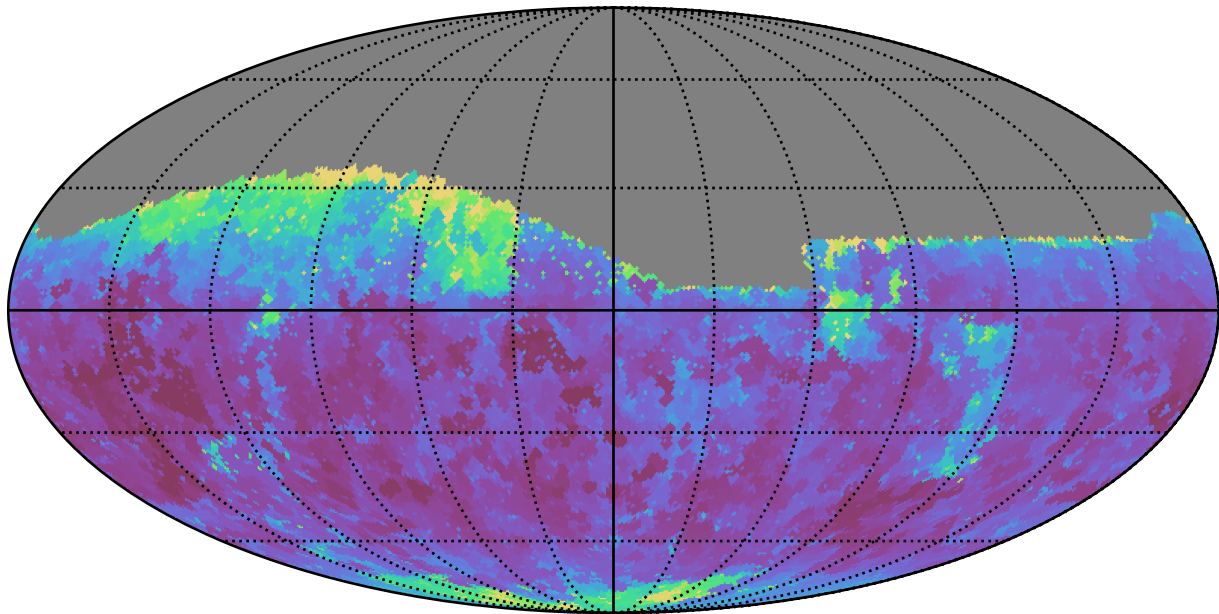
ddf_acor_sf20_lsf30_lsr20_v3.4_10yrs Yr 1 z band: Min seeingEff
