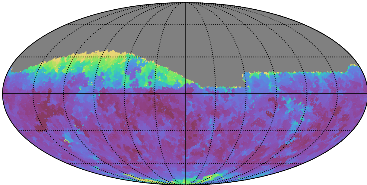
ddf_acor_sf20_lsf30_lsr20_v3.4_10yrs Yr 1 i band: Min seeingEff
