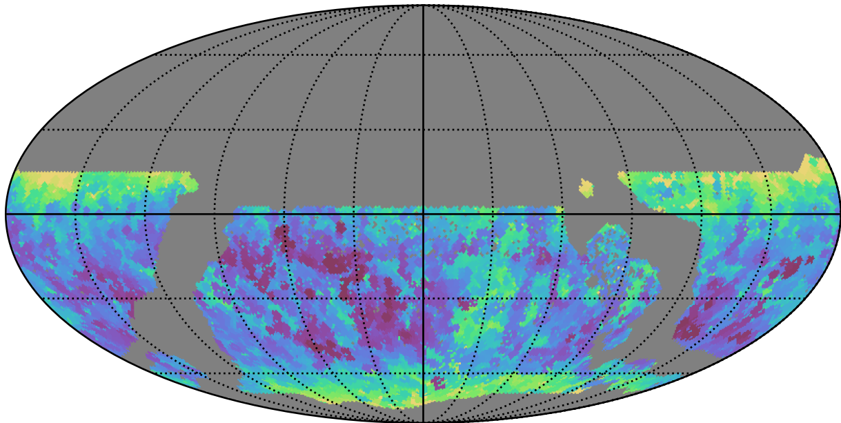
ddf_acor_sf20_lsf30_lsr20_v3.4_10yrs WFD y band: Min seeingEff
