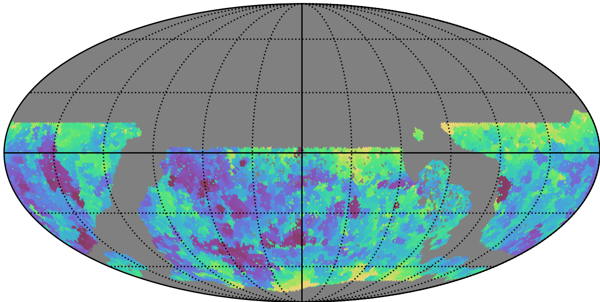
ddf_acor_sf20_lsf30_lsr20_v3.4_10yrs WFD g band: Min seeingEff
