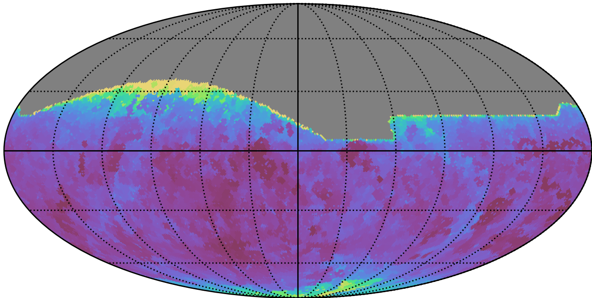
ddf_acor_sf20_lsf30_lsr20_v3.4_10yrs All sky r band: Min seeingEff
