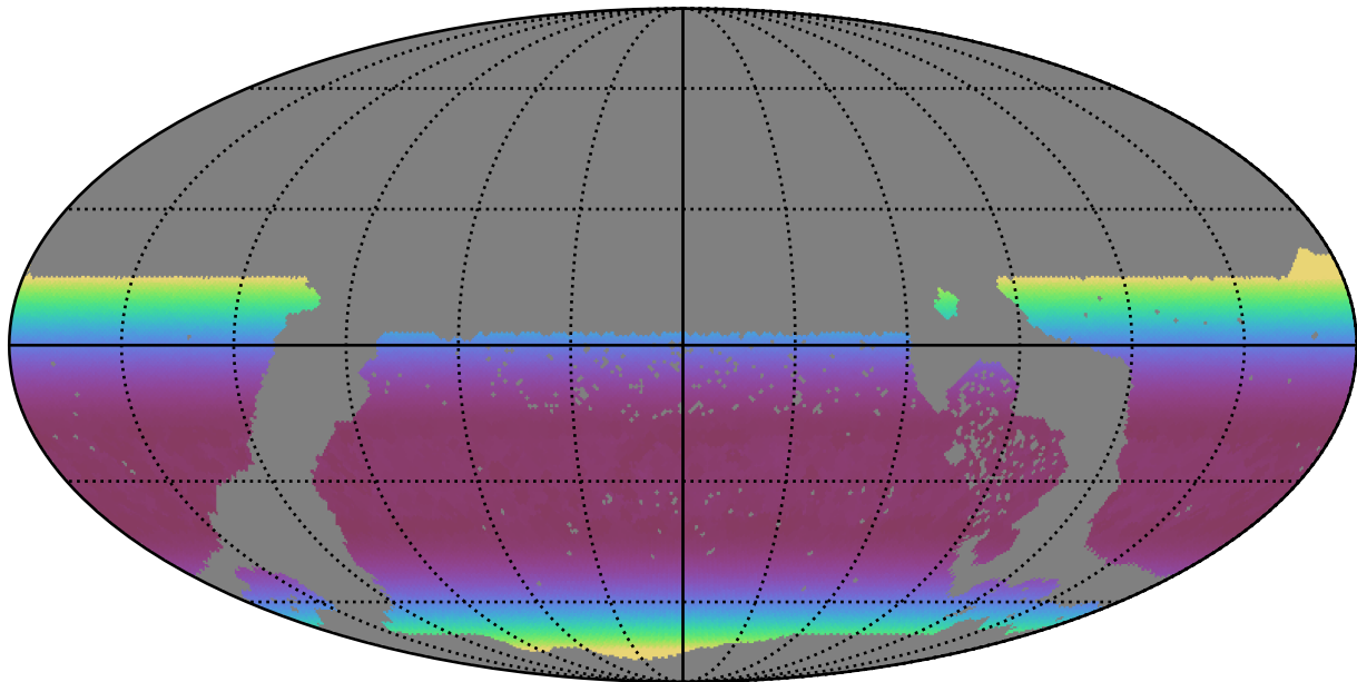
ddf_acor_sf20_lsf30_lsr20_v3.4_10yrs WFD all bands: Min airmass
