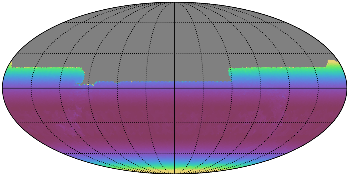
ddf_acor_sf20_lsf30_lsr20_v3.4_10yrs All sky y band: Min airmass
