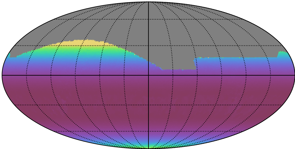
ddf_acor_sf20_lsf30_lsr20_v3.4_10yrs All sky r band: Min airmass
