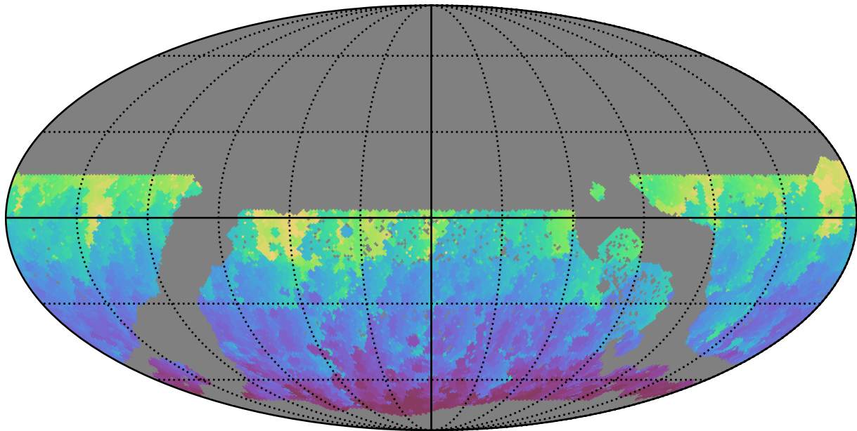
ddf_acor_sf20_lsf30_lsr20_v3.4_10yrs WFD g band: Min HA
