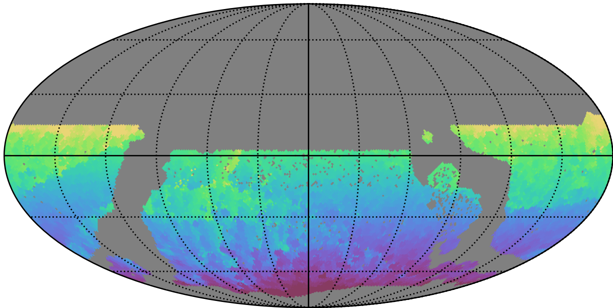
ddf_acor_sf20_lsf30_lsr20_v3.4_10yrs WFD all bands: Min HA
