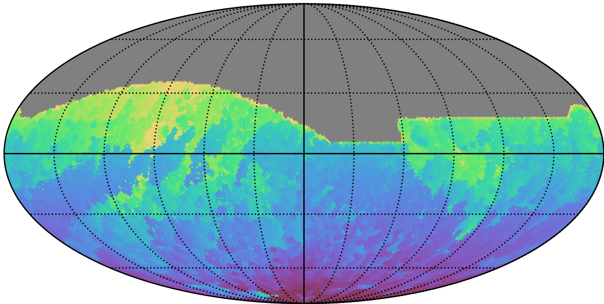
ddf_acor_sf20_lsf30_lsr20_v3.4_10yrs All sky z band: Min HA
