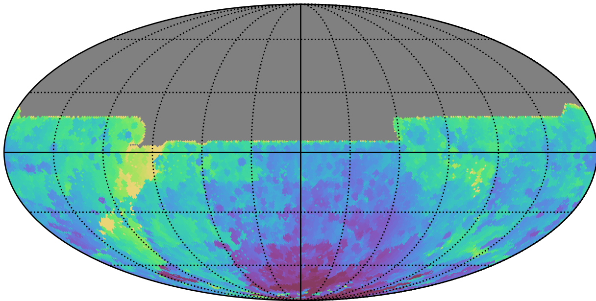
ddf_acor_sf20_lsf30_lsr20_v3.4_10yrs All sky y band: Min HA
