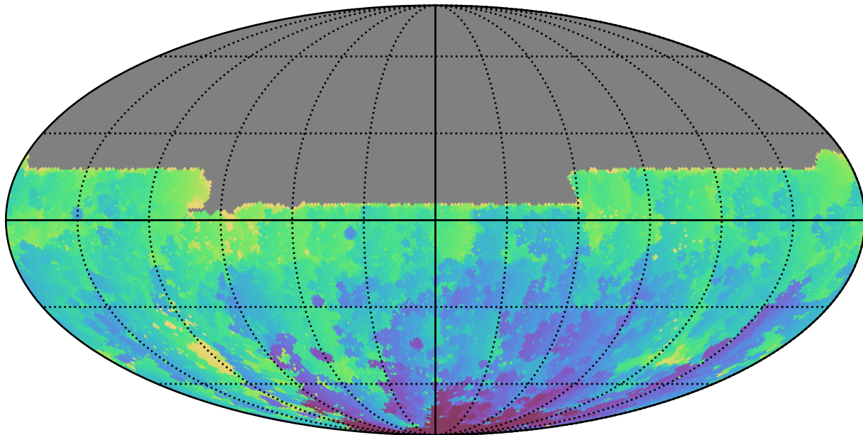
ddf_acor_sf20_lsf30_lsr20_v3.4_10yrs All sky u band: Min HA
