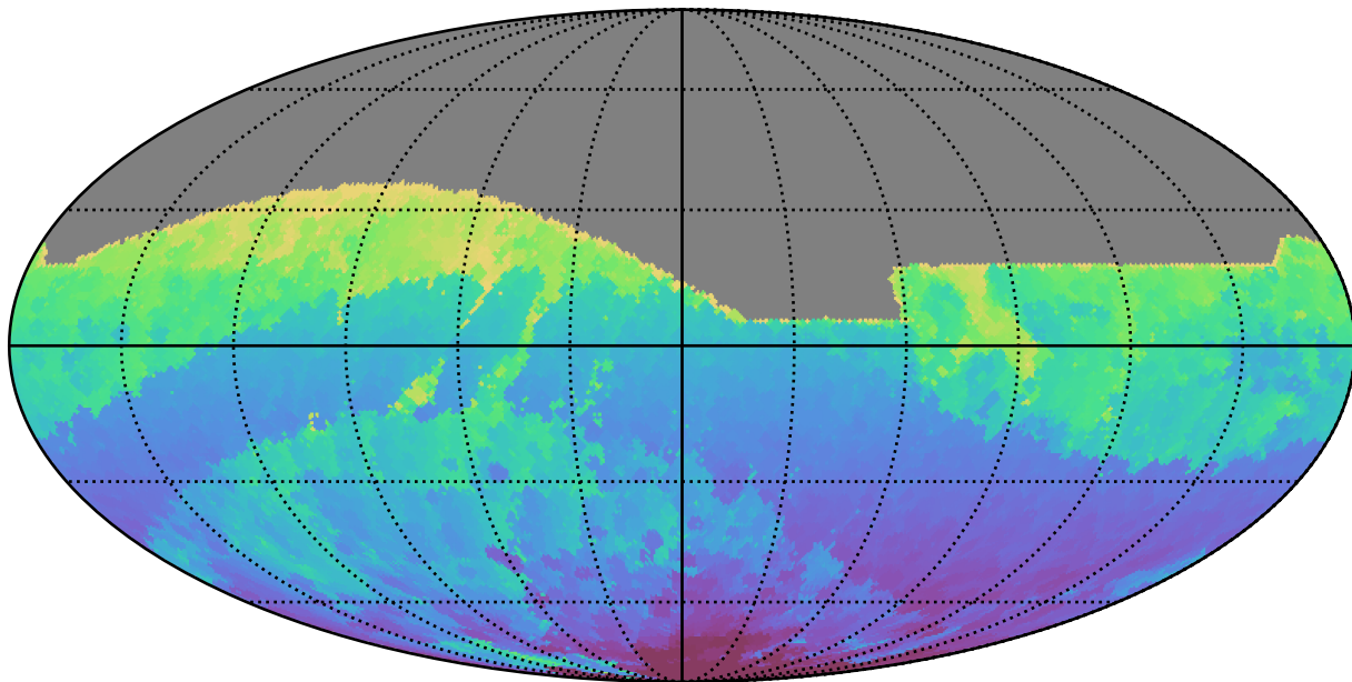
ddf_acor_sf20_lsf30_lsr20_v3.4_10yrs All sky r band: Min HA
