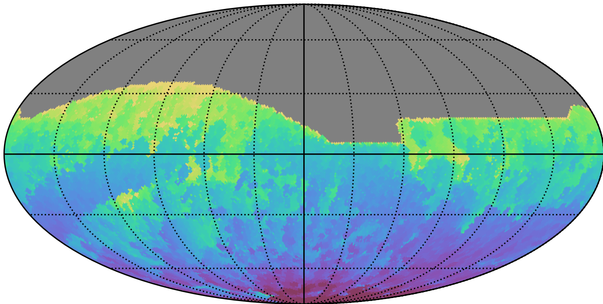
ddf_acor_sf20_lsf30_lsr20_v3.4_10yrs All sky i band: Min HA
