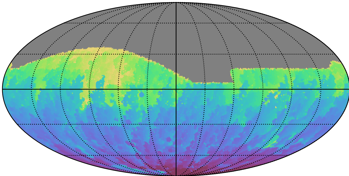
ddf_acor_sf20_lsf30_lsr20_v3.4_10yrs All sky g band: Min HA
