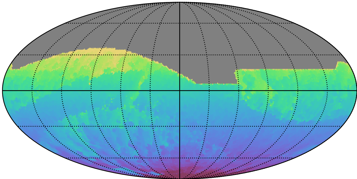
ddf_acor_sf20_lsf30_lsr20_v3.4_10yrs All sky all bands: Min HA
