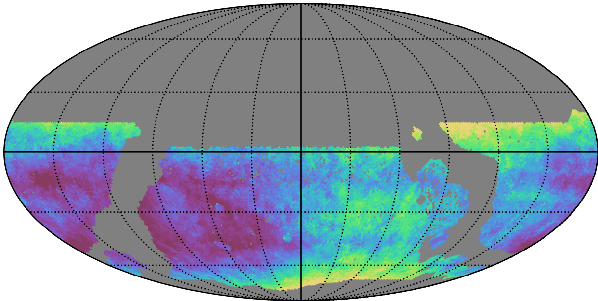
ddf_acor_sf20_lsf30_lsr20_v3.4_10yrs WFD i band: Median seeingEff
