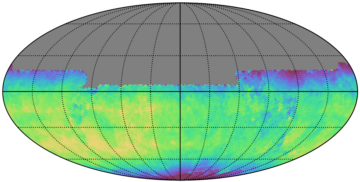
ddf_acor_sf20_lsf30_lsr20_v3.4_10yrs All sky y band: Median fiveSigmaDepth
