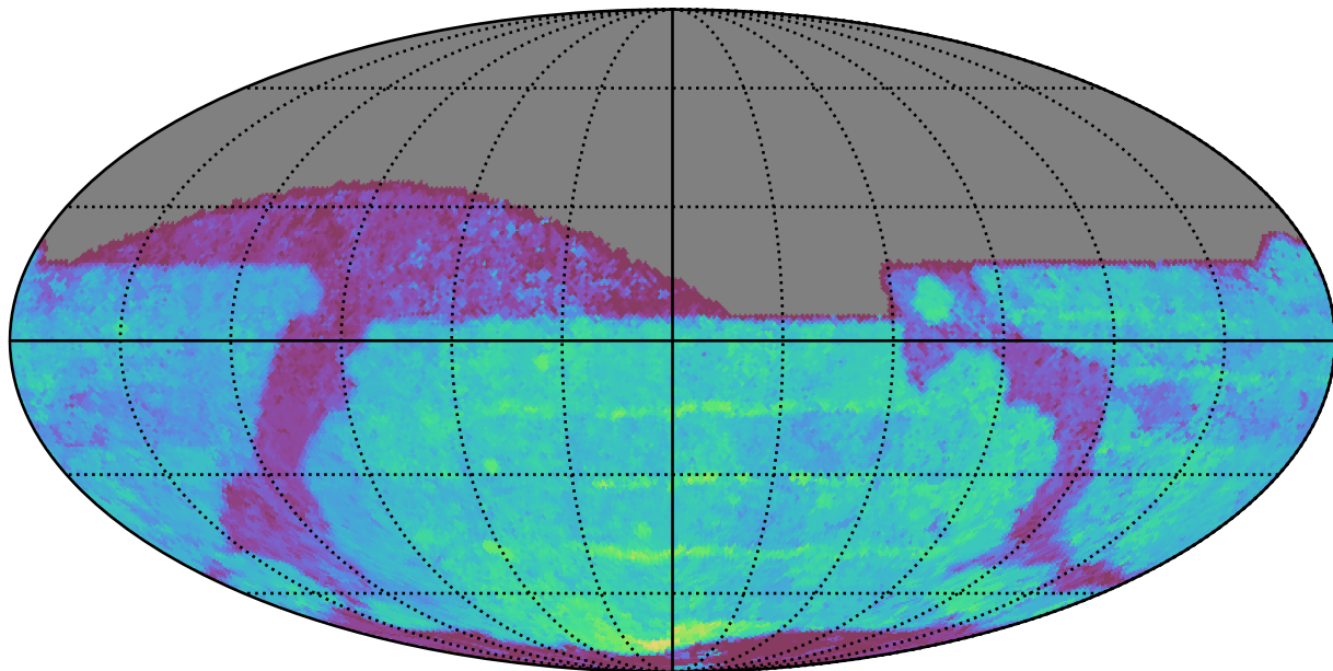
ddf_acor_sf20_lsf30_lsr20_v3.4_10yrs All sky z band: Median Season Length
