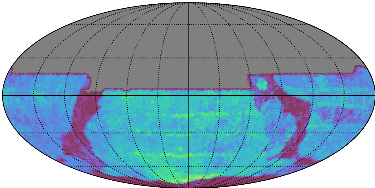
ddf_acor_sf20_lsf30_lsr20_v3.4_10yrs All sky y band: Median Season Length
