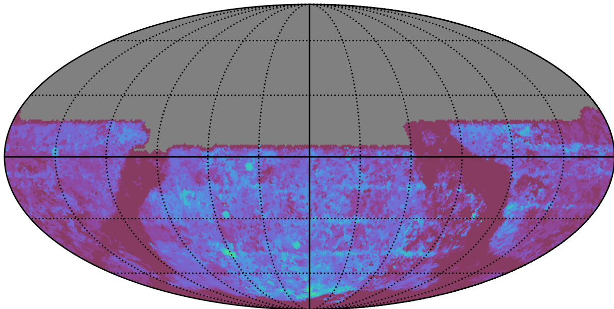
ddf_acor_sf20_ls30_lsr20_v3.4_10yrs All sky u band: Median Season Length
