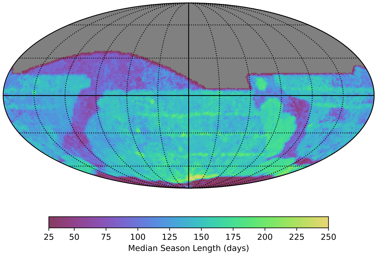
ddf_acor_sf20_lsf30_lsr20_v3.4_10yrs All sky r band: Median Season Length
