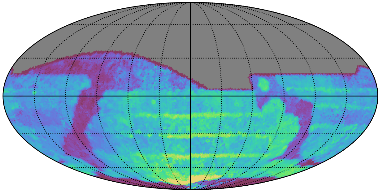
ddf_acor_sf20_lsf30_lsr20_v3.4_10yrs All sky all bands: Median Season Length
