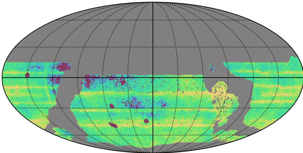
ddf_acor_sf20_lsf30_lsr20_v3.4_10yrs WFD: Median Intra-Night Gap
