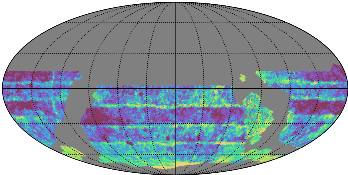
ddf_acor_sf20_lsf30_lsr20_v3.4_10yrs WFD r band: Median Inter-Night Gap
