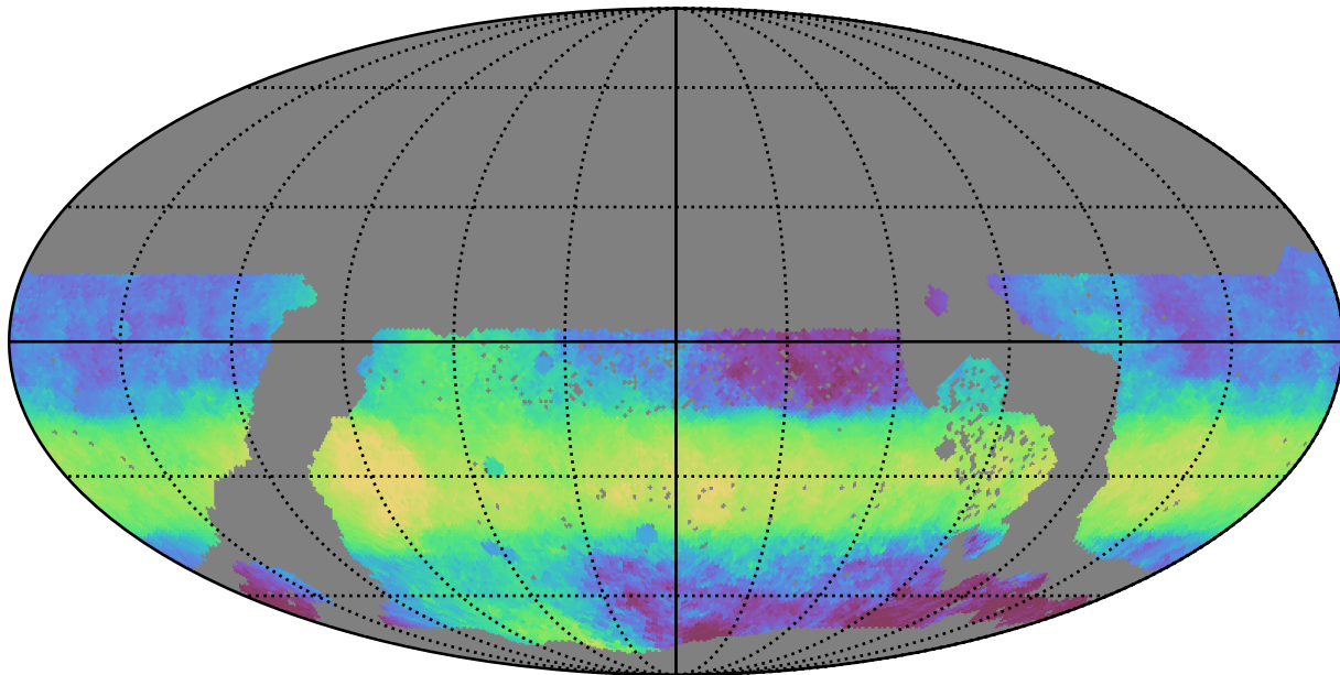
ddf_acor_sf20_lsf30_lsr20_v3.4_10yrs WFD z band: Median HA
