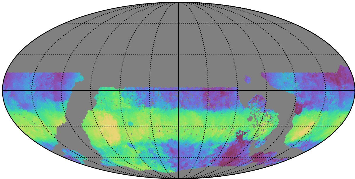
ddf_acor_sf20_lsf30_lsr20_v3.4_10yrs WFD u band: Median HA
