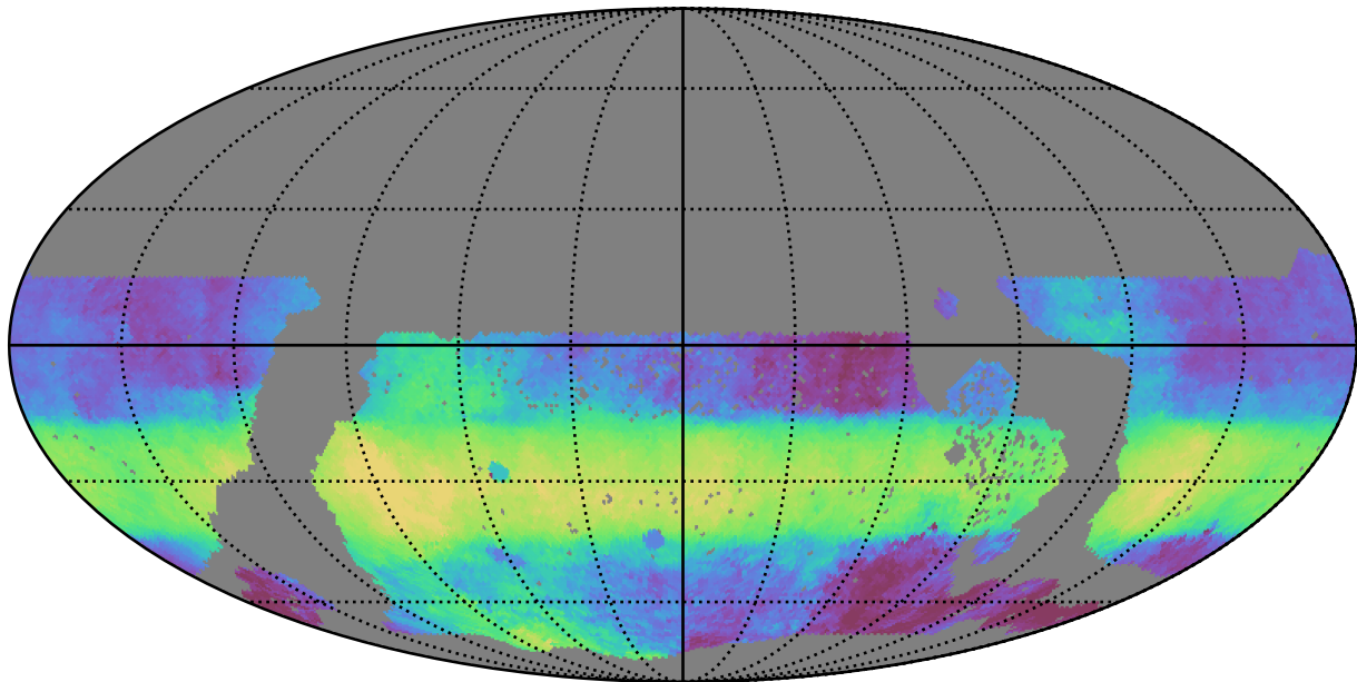
ddf_acor_sf20_lsf30_lsr20_v3.4_10yrs WFD r band: Median HA
