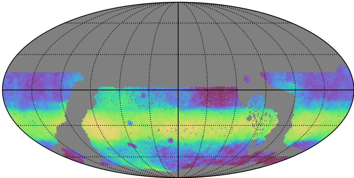
ddf_acor_sf20_lsf30_lsr20_v3.4_10yrs WFD i band: Median HA
