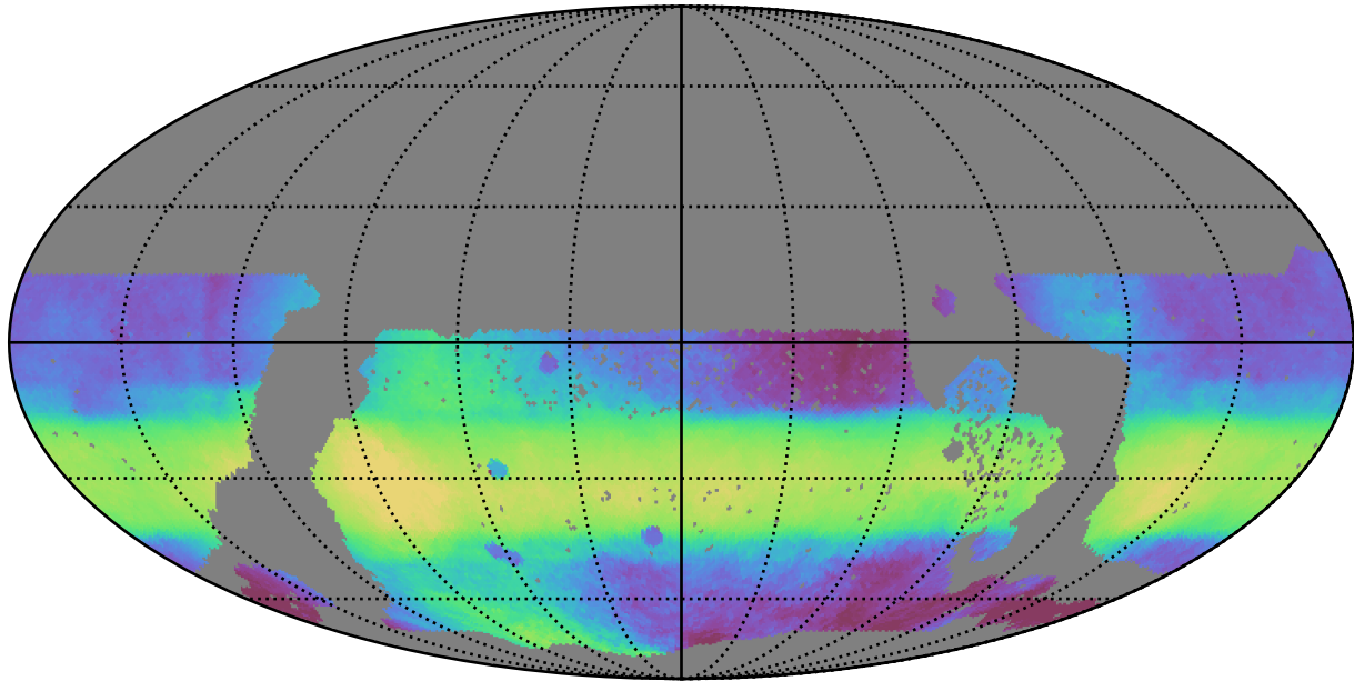
ddf_acor_sf20_lsf30_lsr20_v3.4_10yrs WFD all bands: Median HA
