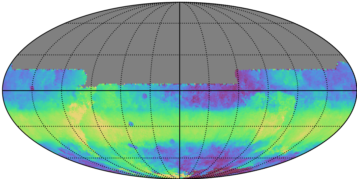
ddf_acor_sf20_lsf30_lsr20_v3.4_10yrs All sky y band: Median HA
