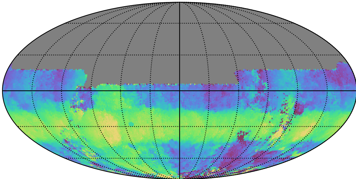
ddf_acor_sf20_lsf30_lsr20_v3.4_10yrs All sky u band: Median HA
