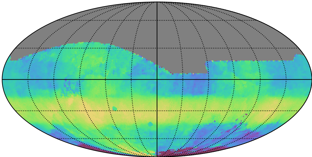
ddf_acor_sf20_lsf30_lsr20_v3.4_10yrs All sky r band: Median HA
