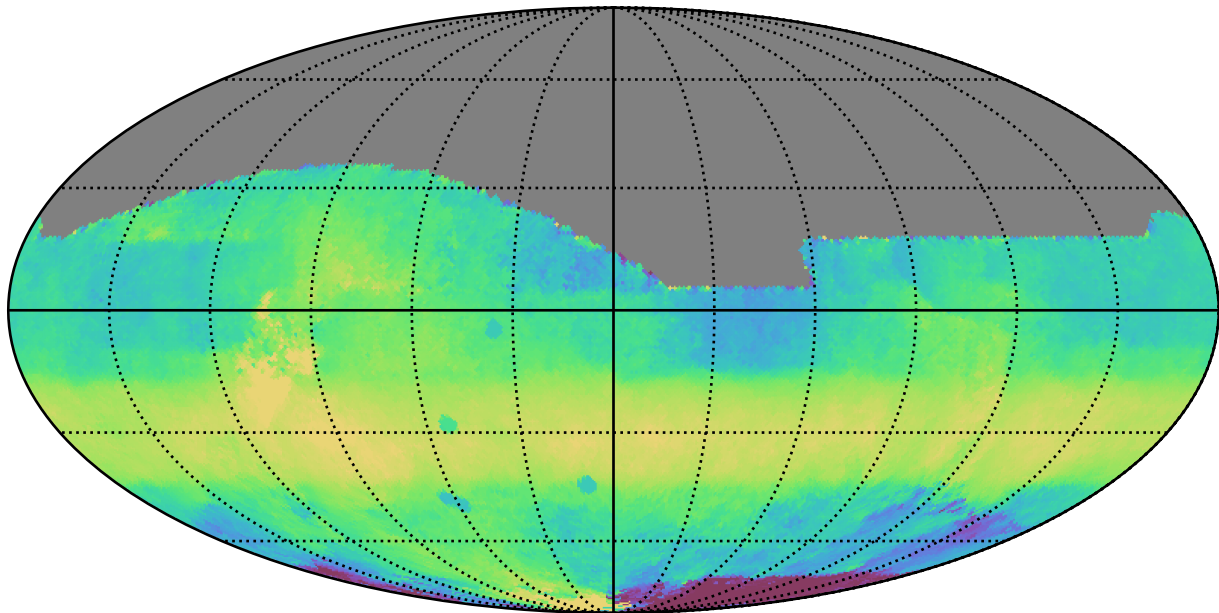
ddf_acor_sf20_lsf30_lsr20_v3.4_10yrs All sky i band: Median HA
