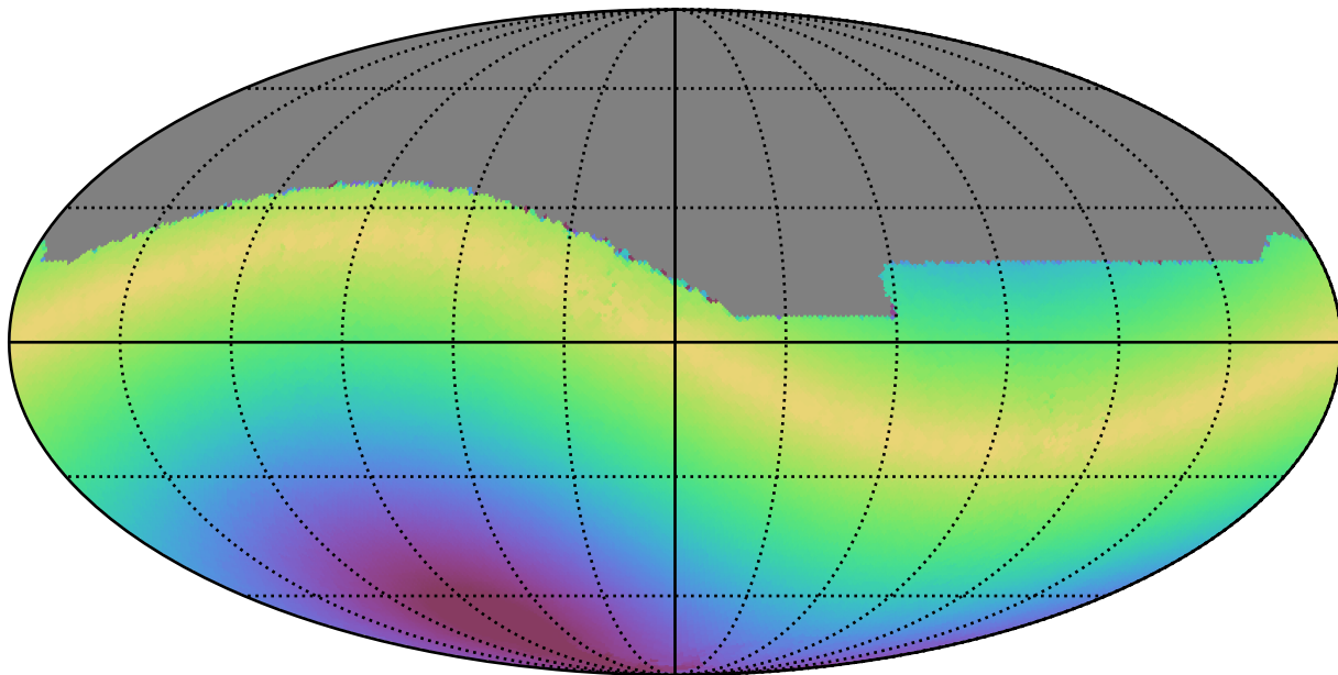
ddf_acor_sf20_lsf30_lsr20_v3.4_10yrs All sky i band: Max solarElong
