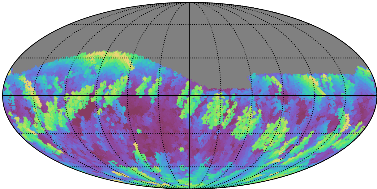
ddf_acor_sf20_lsf30_lsr20_v3.4_10yrs Yr 1 r band: Max airmass
