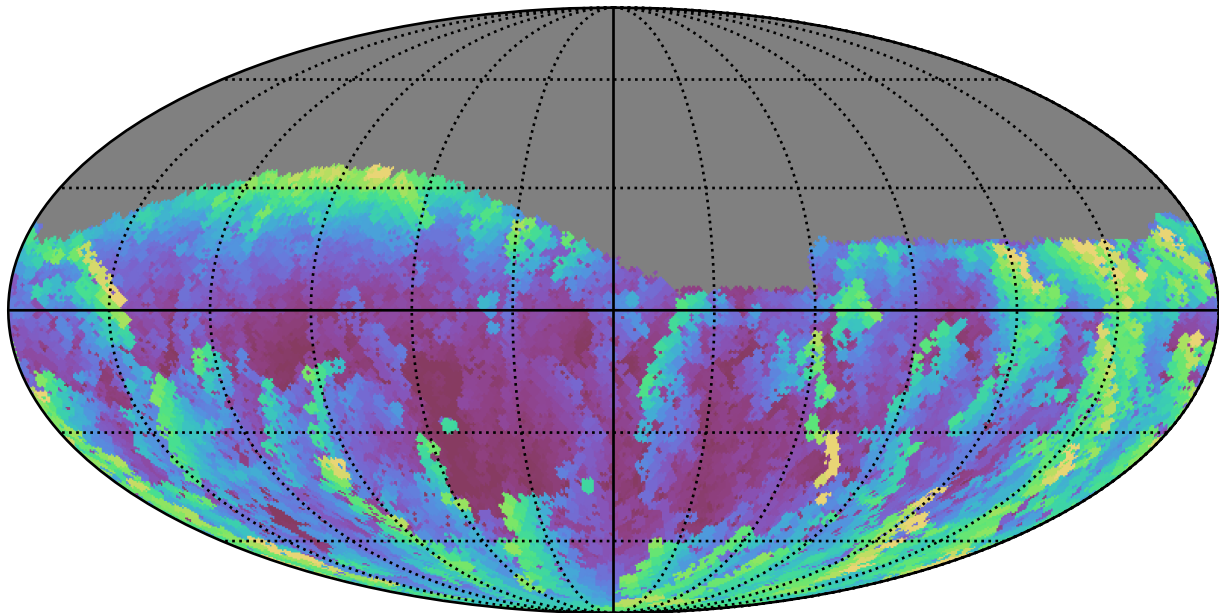
ddf_acor_sf20_lsf30_lsr20_v3.4_10yrs Yr 1 g band: Max airmass
