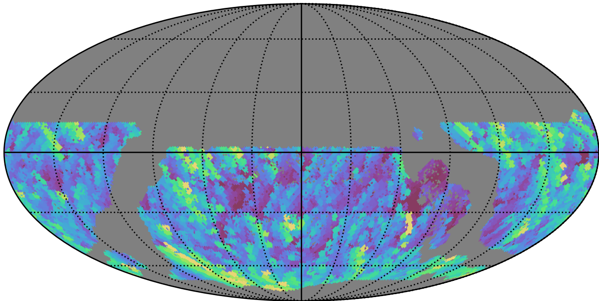
ddf_acor_sf20_lsf30_lsr20_v3.4_10yrs WFD g band: Max airmass
