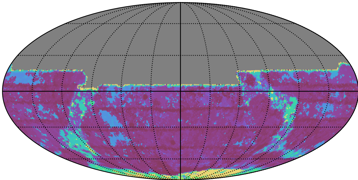
ddf_acor_sf20_lsf30_lsr20_v3.4_10yrs All sky y band: Max Inter-Night Gap
