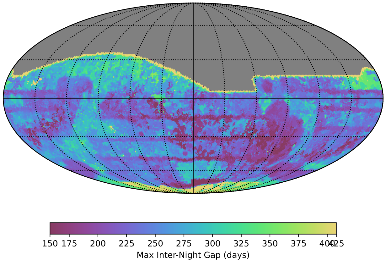
ddf_acor_sf20_lsf30_lsr20_v3.4_10yrs All sky all bands: Max Inter-Night Gap
