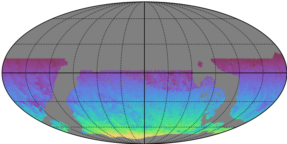
ddf_acor_sf20_lsf30_lsr20_v3.4_10yrs WFD all bands: Max HA
