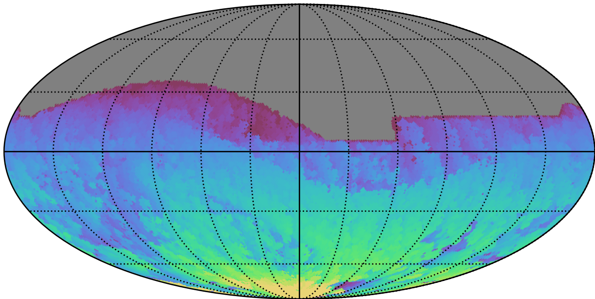
ddf_acor_sf20_lsf30_lsr20_v3.4_10yrs All sky z band: Max HA
