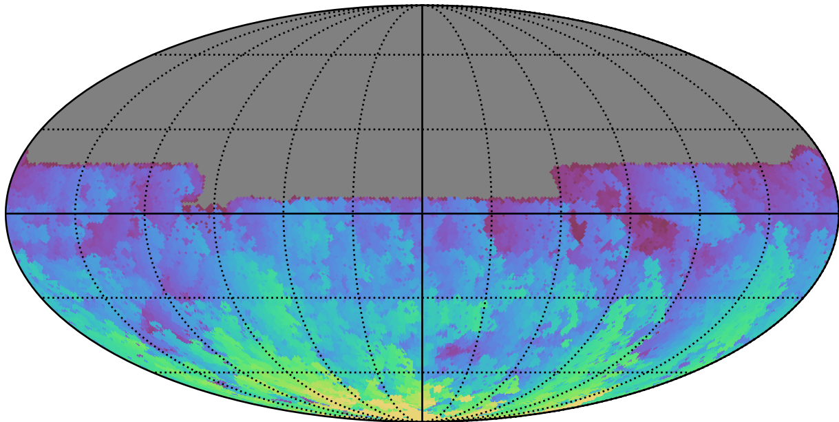
ddf_acor_sf20_lsf30_lsr20_v3.4_10yrs All sky u band: Max HA
