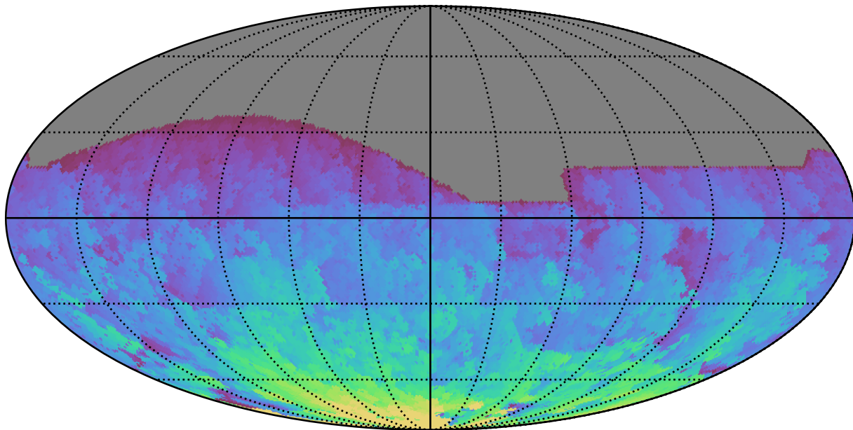
ddf_acor_sf20_lsf30_lsr20_v3.4_10yrs All sky r band: Max HA
