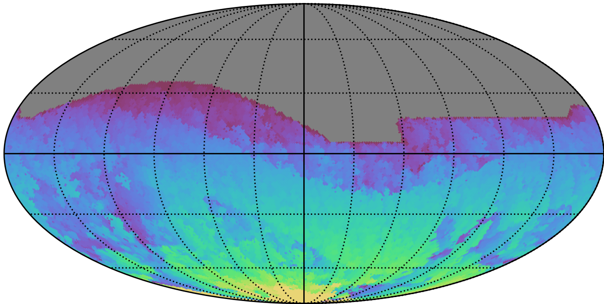
ddf_acor_sf20_lsf30_lsr20_v3.4_10yrs All sky i band: Max HA
